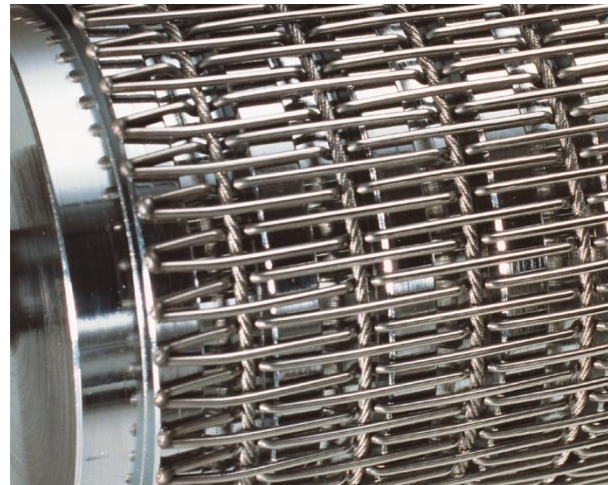
Picture 4-5: V-crims on the underside of the mesh ensure optimal and reliable self-tracking.
