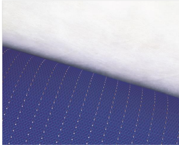
Picture 2: Low fibre breakdown and good separation behaviour through antistatic CONDUCTO® with bronze wires.
